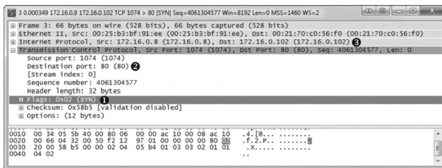
Figure 8-22: TCP SYN packet sent from one internal host to another
