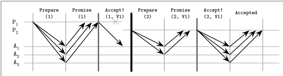
Figure 14-4. Paxos failure scenario: proposer failure, deciding on the old value
