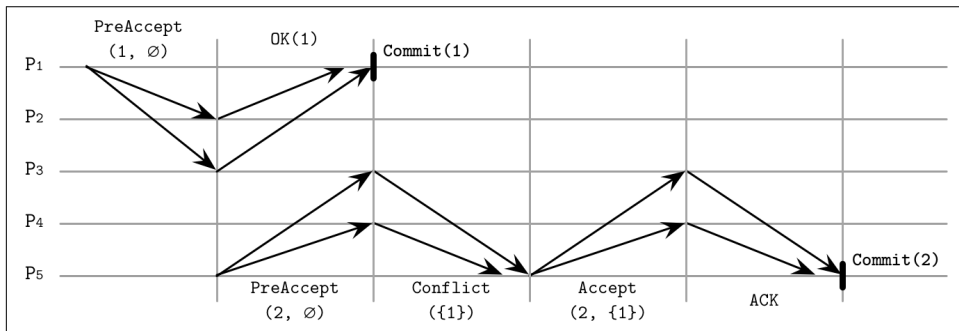
Figure 14-8. EPaxos algorithm run
