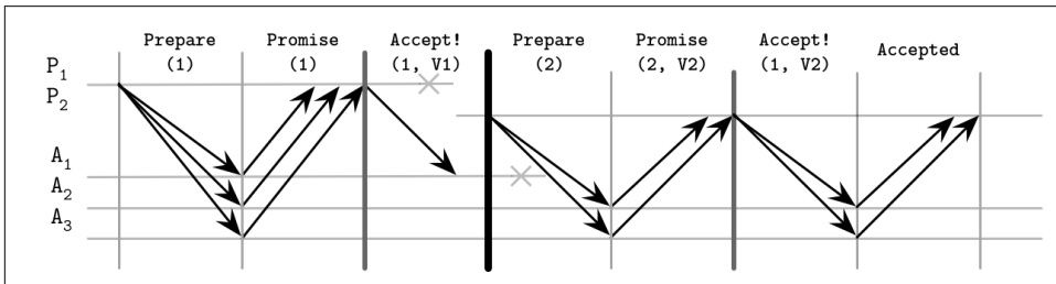
Figure 14-6. Paxos failure scenario: proposer failure, followed by the acceptor failure
