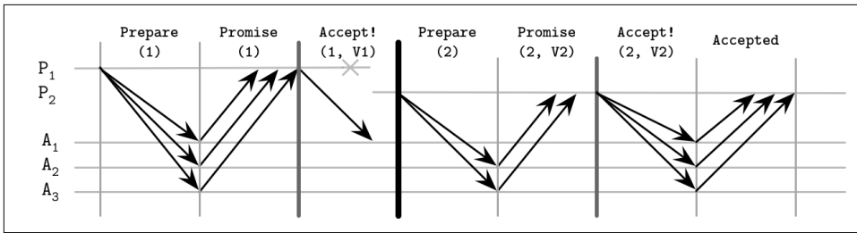
Figure 14-5. Paxos failure scenario: proposer failure, deciding on the new value
