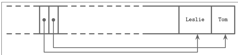
Figure 3-7. Records appended in random order: Tom , Leslie
