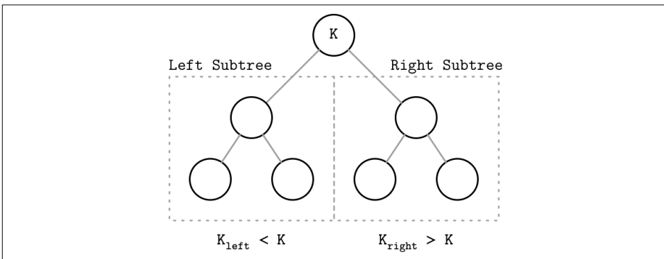
Figure 2-2. Binary tree node invariants
